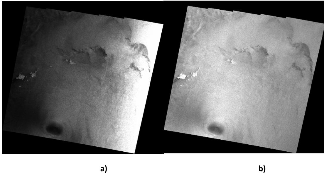
Figure A3.2 Sentinel-1 EW [ORB] product. a) ORB intensity (Sigma-Nought); b) Intensity compensated with the “Mean Wind-Normalised Backscatter Measurement” (i.e., not Sigma-Nought) and geocoded. Processing: G. Hajduch (CLS).
