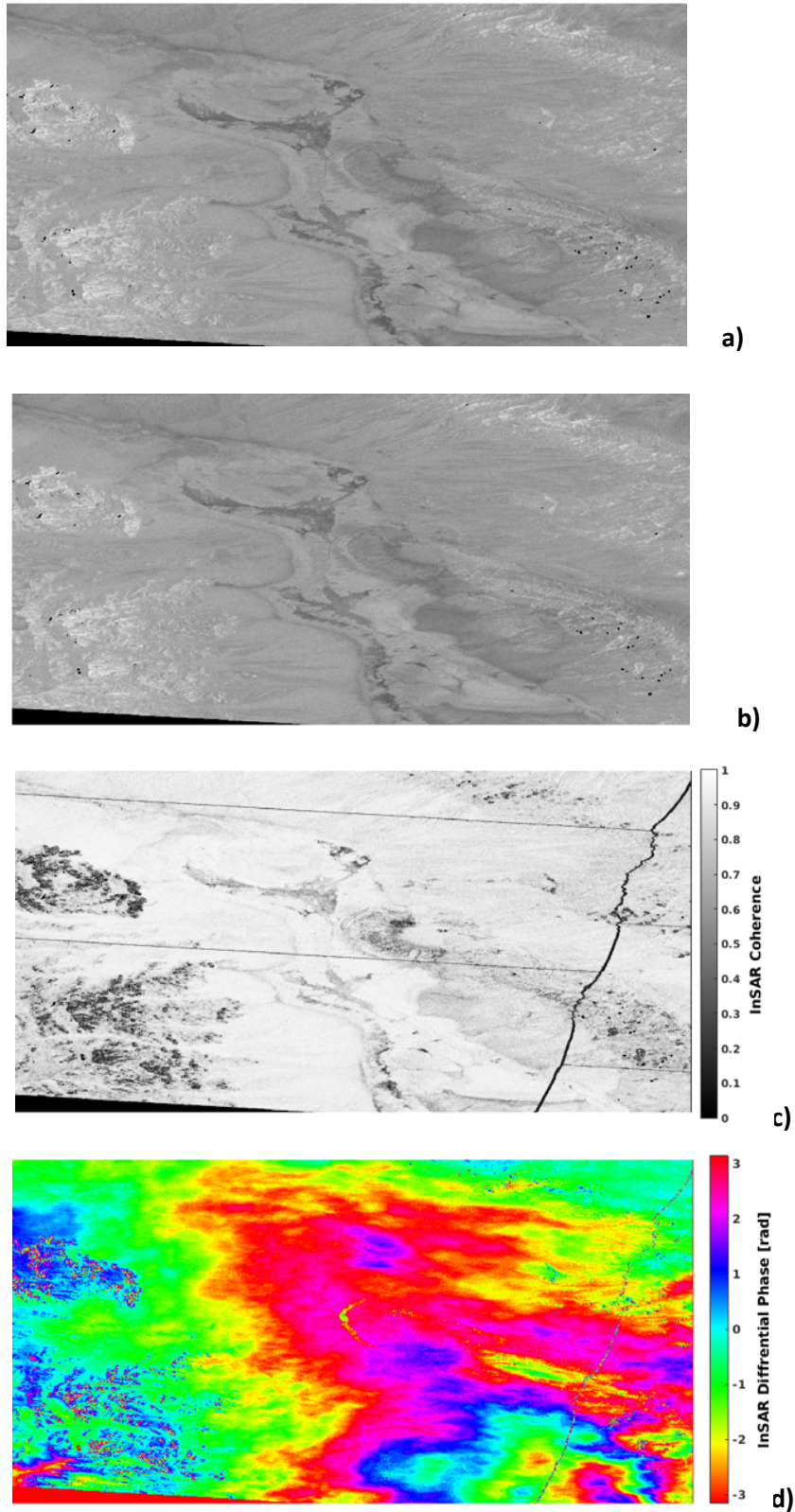
Figure A4.1 Sentinel-1 [GSLC] products example over Death Valley National Park, California, US. a) GSLC1: Intensity data of the first [GSLC] product (2017-05-27); b) GSLC2: Intensity data of the second [GSLC] product (2017-06-08); c) InSAR coherence map generated directly from A4.1a) and b); d) InSAR differential phase map generated directly from A4.1a) and b).
